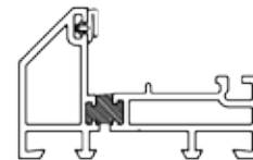
44MM ALUMINIUM THRESHOLD (BEVELLED)
